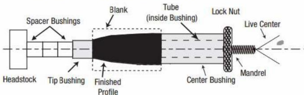
DIAGRAM C - Turning Profile To Bushings
