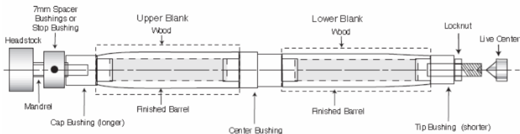
Diagram C - Turning the Blanks
