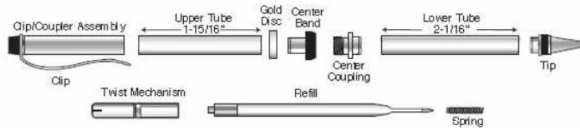
Diagram B - Parts List Pencil
